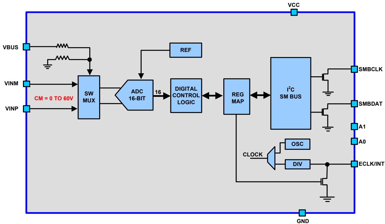
FIGURE 2. BLOCK DIAGRAM
