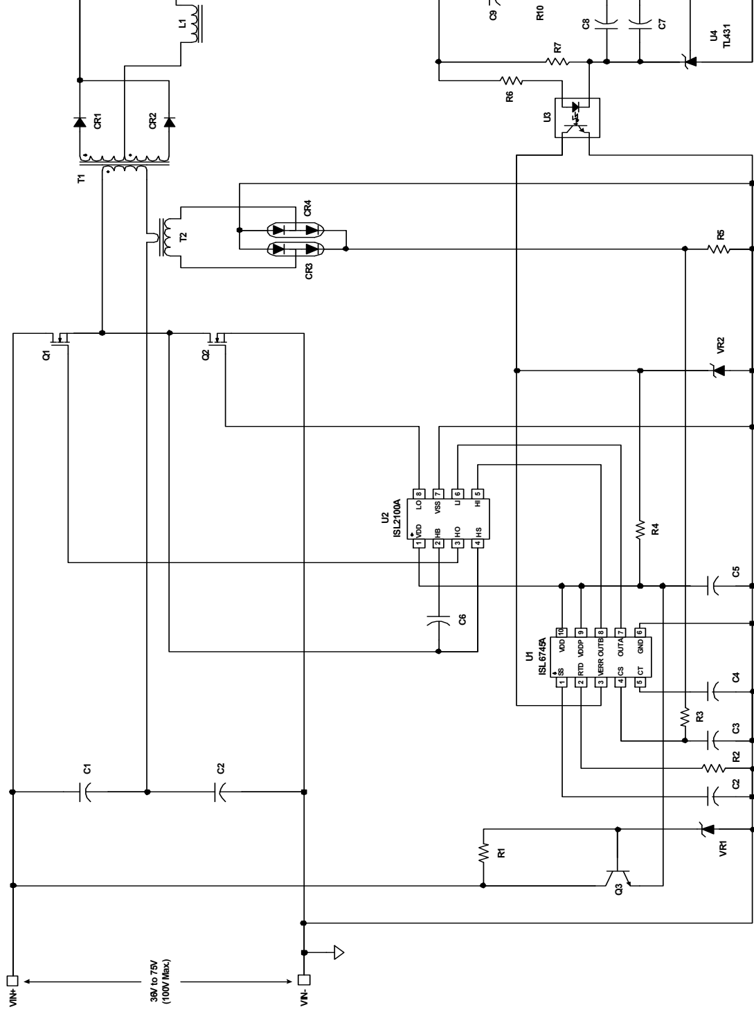
Figure 2. Typical Application
