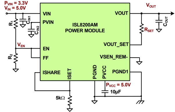
FIGURE 22. 3.3V OPERATION
