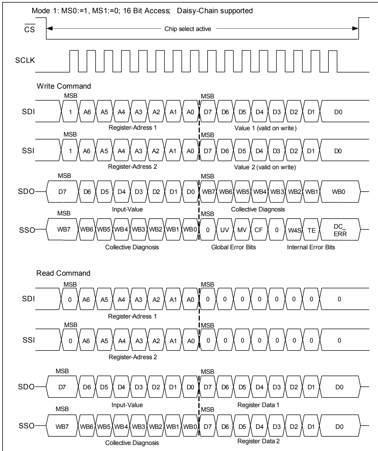
Figure 25 SPI Mode 1
