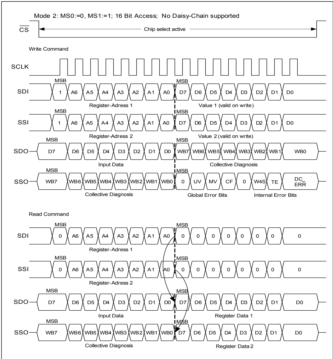
Figure 26 SPI Mode 2
