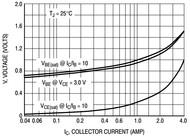
Figure 9. "On" Voltages
