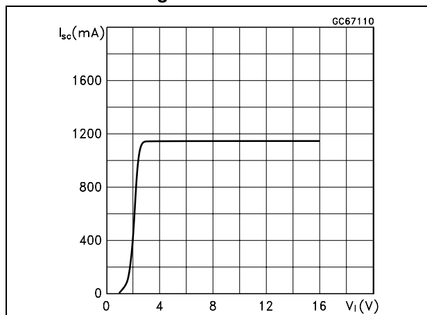
Figure 7. Short circuit current vs input voltage
