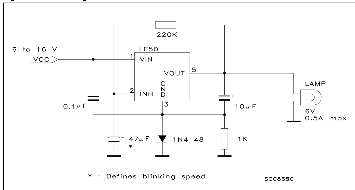
Figure 14. Low voltage bulb blinker
