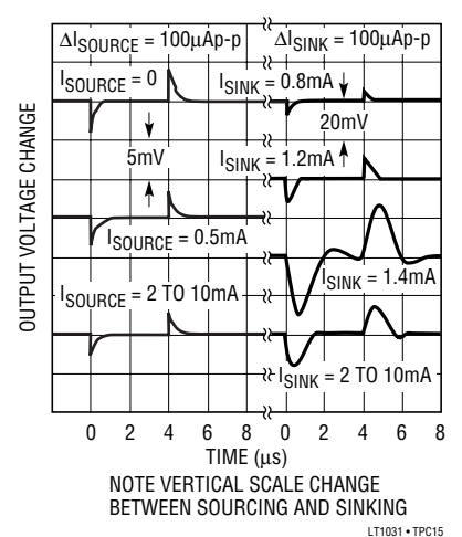
Load Transient Response C_{\text{LOAD}} = 1000\text{pF}
