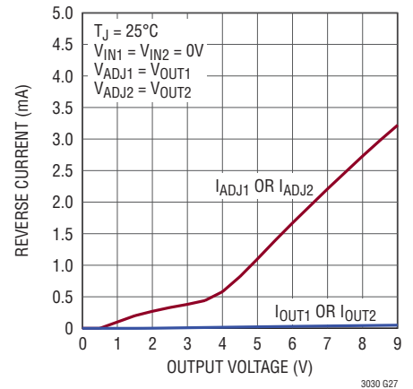
Reverse Current
