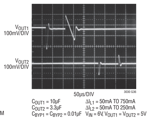
Channel-to-Channel Isolation
