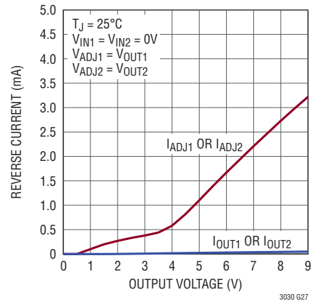
Reverse Current
