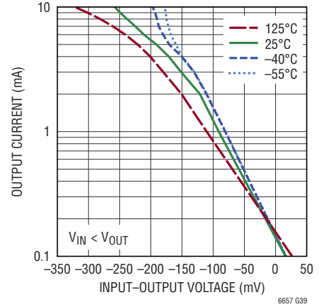
5V Minimum V_{IN} to V_{OUT} Differential (Sinking)
