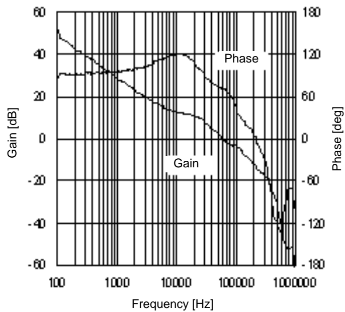
Figure 44. Gain vs Frequency 9 ( V_{CC}=10V , I_o=900mA )
