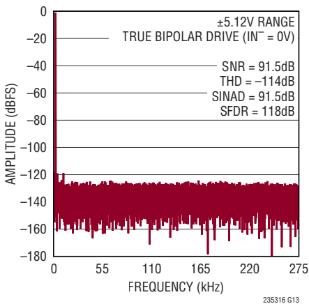
32k Point FFT f_{SAMPL} = 550\text{ksps} , f_{IN} = 2\text{kHz}
