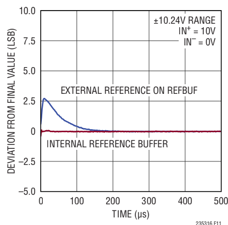
Figure 11. Burst Conversion Response of the LTC2353-16, f_{\text{SMPL}} = 550\text{ksps}
