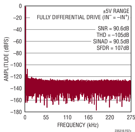
Figure 7c. IN + /IN - = 450mV 200Hz Fully Differential Sine, 0V ≤ V CM ≤ 24V, 32k Point FFT, f SAMPL = 550kps. Circuit Shown in Figure 7a
