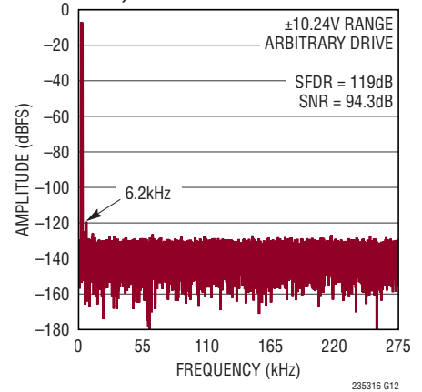
32k Point Arbitrary Two-Tone FFT f_{SAMPL} = 550\text{ksps} , IN^+ = -7\text{dBFS} 2kHz Sine, IN^- = -7\text{dBFS} 3.1kHz Sine
