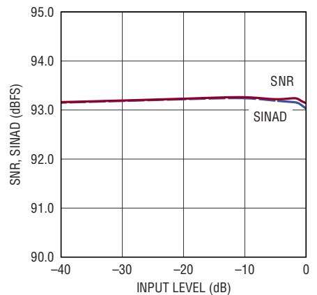
SNR, SINAD vs Input Level, f_{\text{IN}} = 1\text{kHz}
