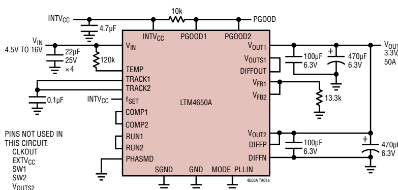
50A, 3.3V Output DC/DC \mu Module Regulator
