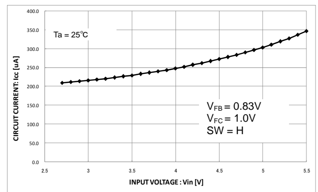
Fig.23 Circuit current-power-supply voltage characteristic
