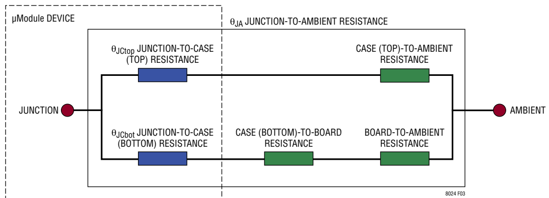
Figure 3. Graphical Approximation of the Thermal Coefficients, Including JEESD51-12 Terms
