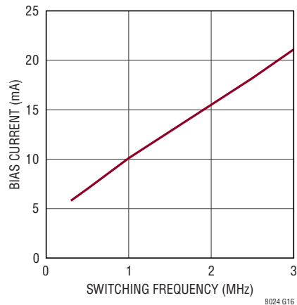
BIAS Current vs Frequency 12\text{V}_{IN} , 3.3\text{V}_{OUT} , 1A Load SYNC Floating
