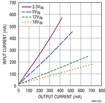
Input Current vs Output Current, -3.3V_{OUT} Inverting Converter
