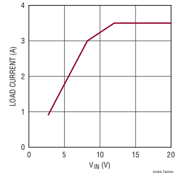
Maximum Load Current vs V IN
