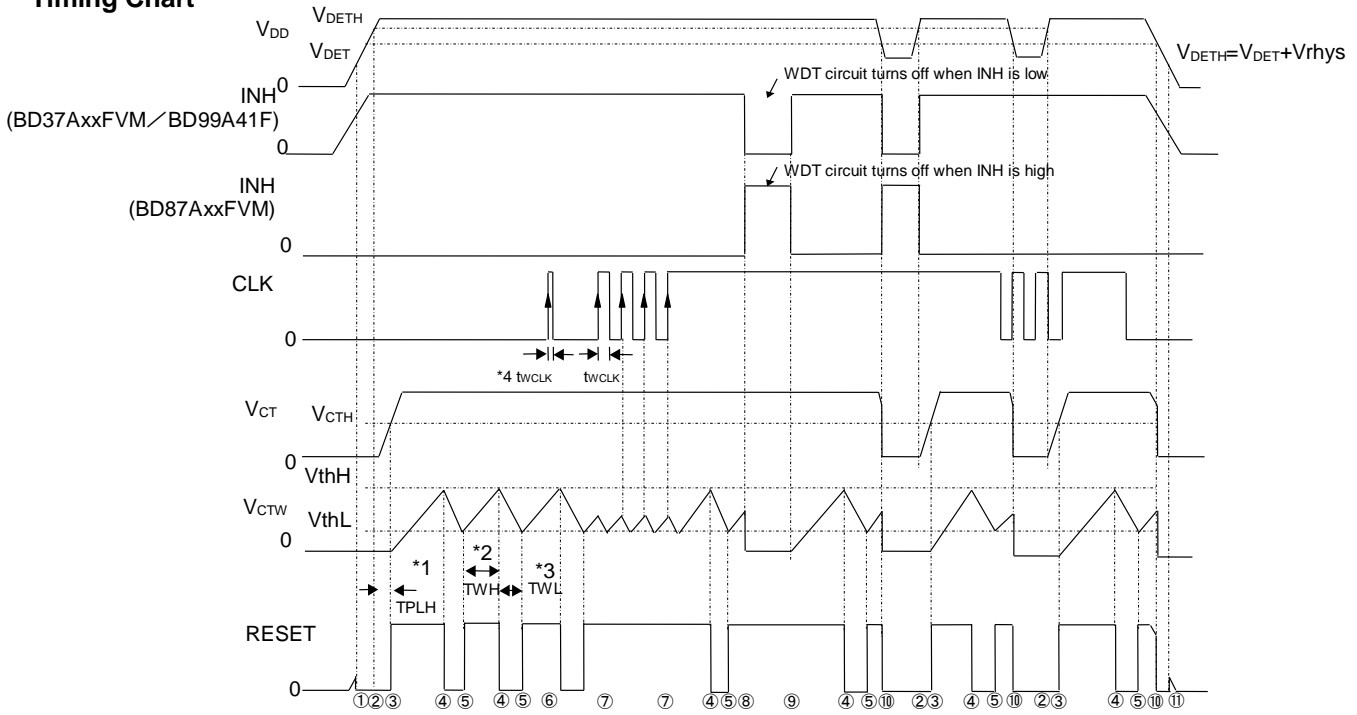
Figure 15. Timing Chart
