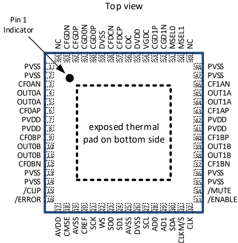
Figure 4-1 Pinout MA12070P
