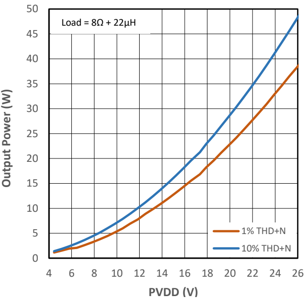
Figure 11-22 Output Power vs PVDD for PMP1
