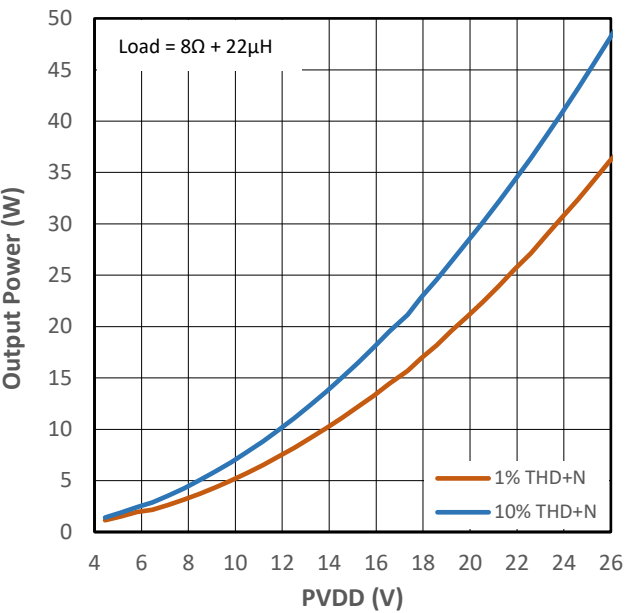
Figure 11-21 Output Power vs PVDD for PMP0
