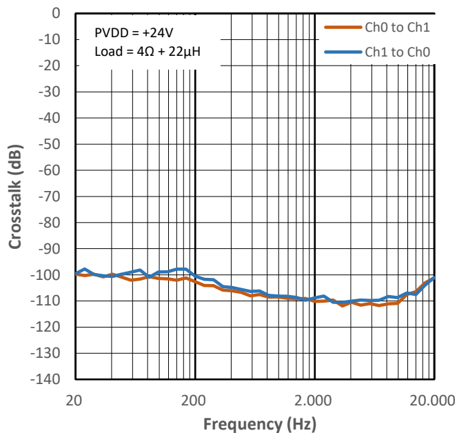
Figure 12-28 Crosstalk vs Frequency for PMP4
