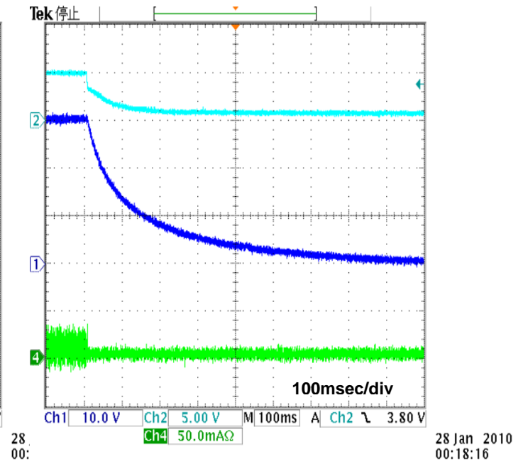
Fig6. ENTERING SHUTDOWN (Condition: Vin=5V, VOUT=31V, Iload=0mA)
