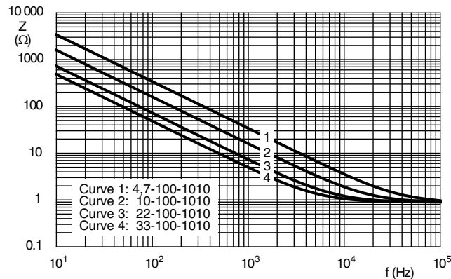
Fig. 15 - Typical impedance Z as a function of frequency at 20 °C
