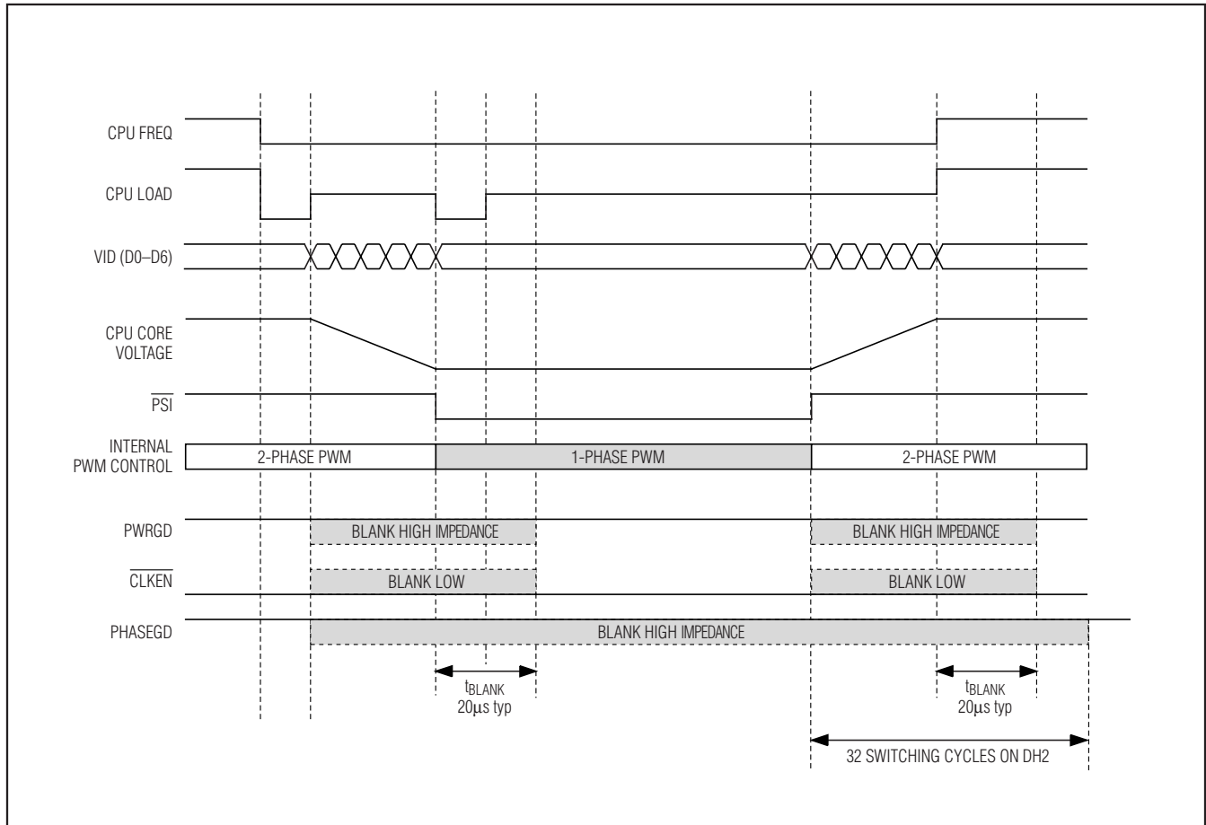
Figure 8. \overline{\text{PSI}} Transition
