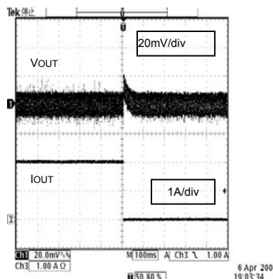
Fig.11 Load response 1
