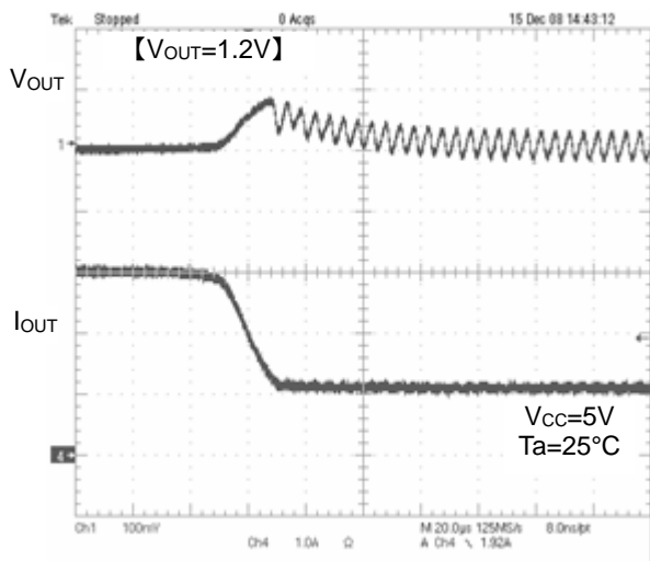
Figure 18. Transient Response (Io=3A to 1A, 10μs)
