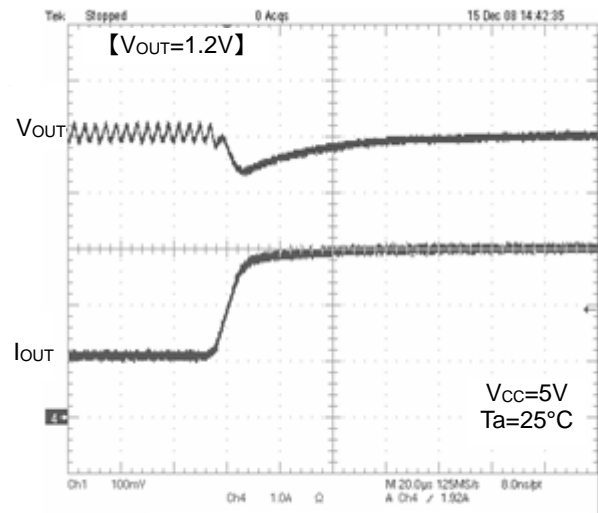
Figure 17. Transient Response (Io=1A to 3A, 10μs)
