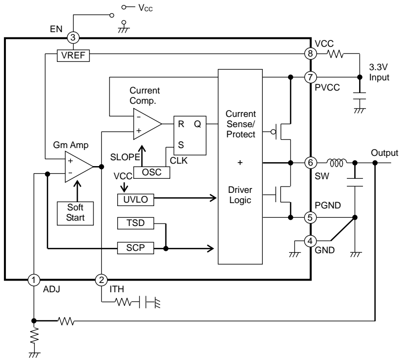
Figure 3. Block Diagram
