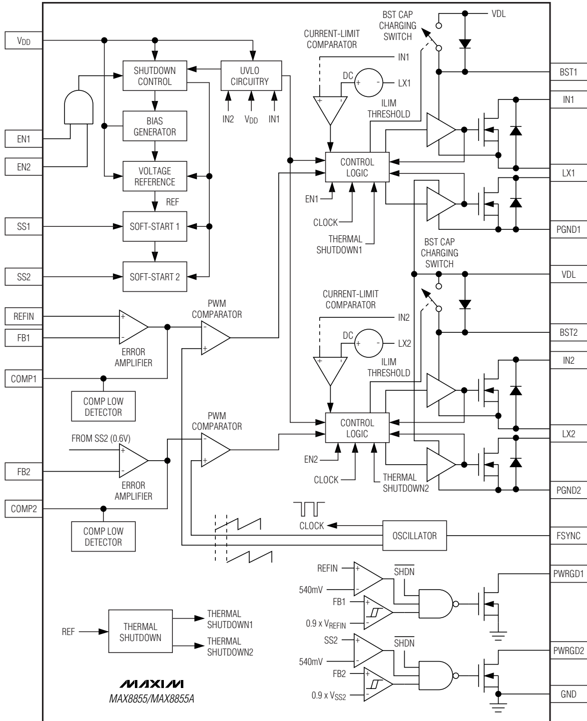
Figure 1. Functional Diagram
