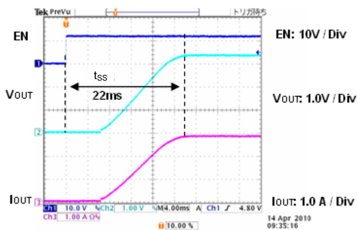
Figure 17. Start-Up Waveform (VIN= 12V, VOUT= 3.3V, L= 10μH, C SS = 0.1μF)
