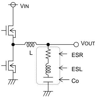
Output capacitor
