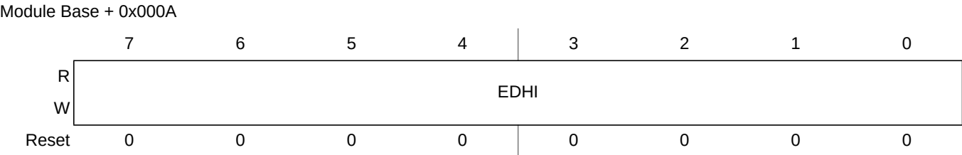
Figure 3-15. EEPROM Data High Register (EDATAHI)
