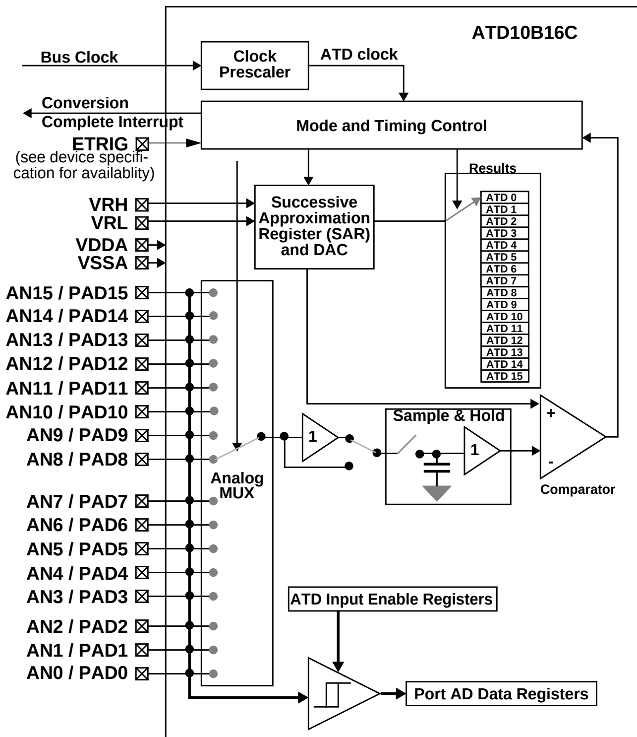
Figure 7-1. ATD10B16C Block Diagram
