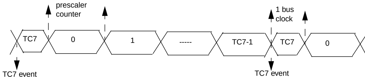
Figure 13-29. The TCNT cycle diagram under TCRE=1 condition
