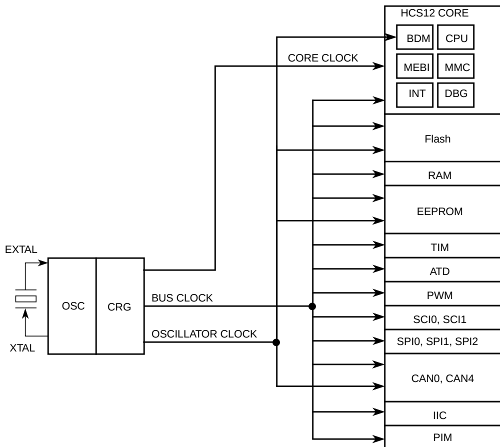
Figure 1-12. Clock Connections
