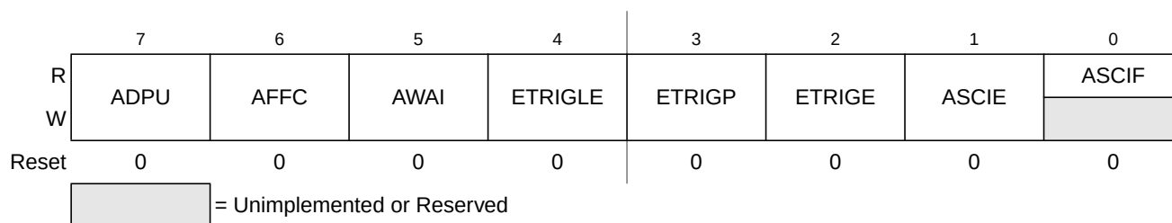
Figure 7-5. ATD Control Register 2 (ATDCTL2)
