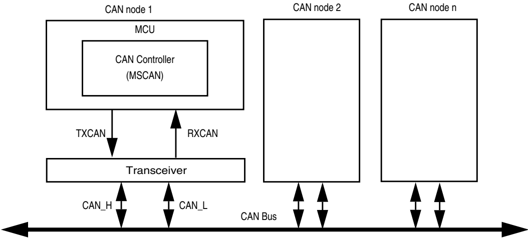
Figure 9-2. CAN System
