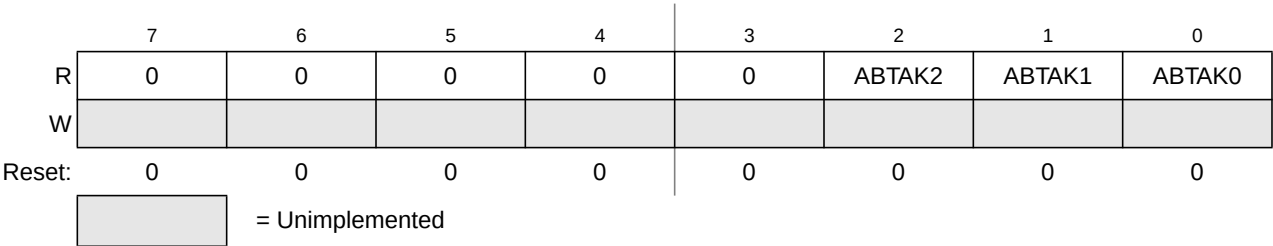
Figure 9-13. MSCAN Transmitter Message Abort Acknowledge Register (CANTAAB)
