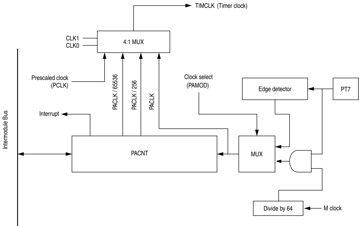
Figure 13-2. 16-Bit Pulse Accumulator Block Diagram
