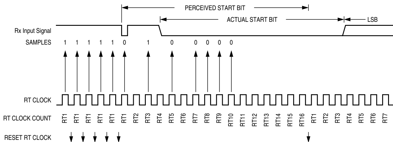
In Figure 10-15 , verification sample at RT3 is high. The RT3 sample sets the noise flag. Although the perceived bit time is misaligned, the data samples RT8, RT9, and RT10 are within the bit time and data recovery is successful.
