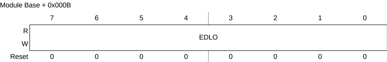
Figure 3-16. EEPROM Data Low Register (EDATALO)
