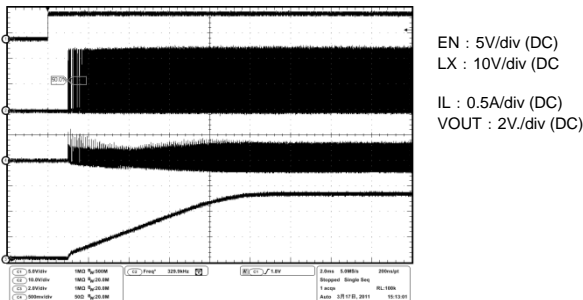
Figure 29. startup Waveform
