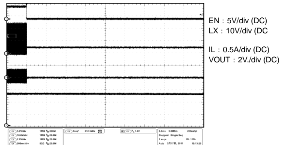
Figure 30. Stop Waveform
