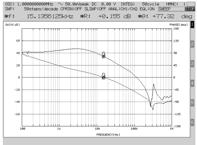
Figure 34. Frequency Response Characteristics ( I_o=3.0A )
