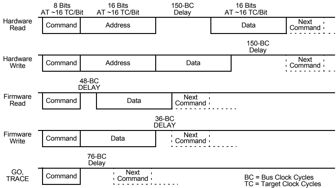
Figure 59. BDM Command Structure
