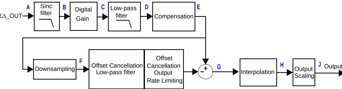
Figure 15. Signal-chain diagram
