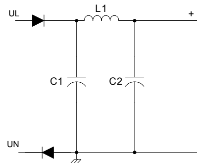
Figure 10: Half-Wave Rectifier
