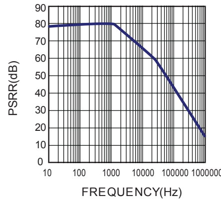
PSRR vs. Frequency I_{OUT}=10mA
