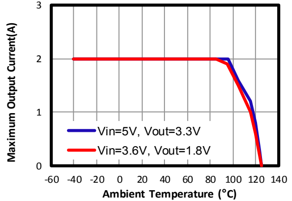
Output Current Derating vs. Ambient Temperature T_J \leq 125^\circ C
