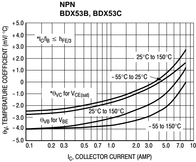
Figure 11. Temperature Coefficients
