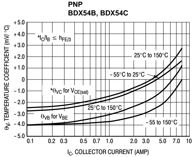
Figure 11. Temperature Coefficients
