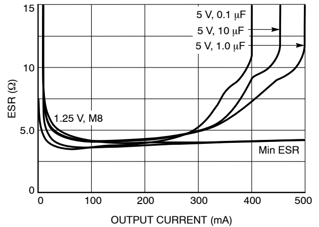
Figure 28. Output Current vs. ESR
