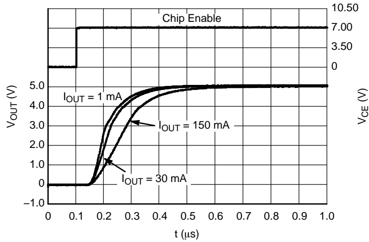
Figure 43. Start-up, 5.0 V Version, V_{IN} = 7.0 \text{ V}
