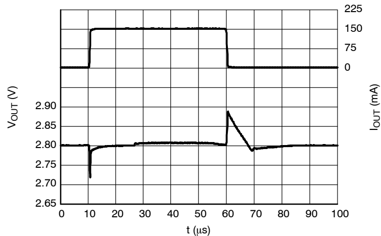
Figure 45. Load Transients, 2.8 V Version, I_{OUT} = 1 - 150 mA, t_R = t_F = 0.5 \mu s, V_{IN} = 3.8 V
