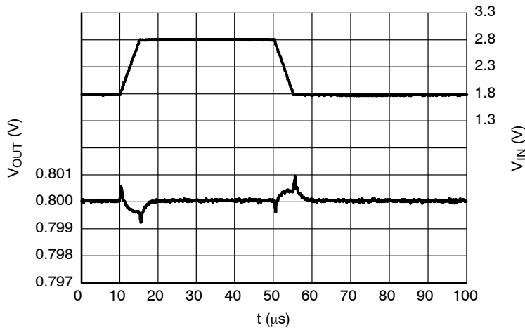
Figure 35. Line Transients, 0.8 V Version, t_R = t_F = 5 \mu\text{s} , I_{\text{OUT}} = 30 \text{ mA}
