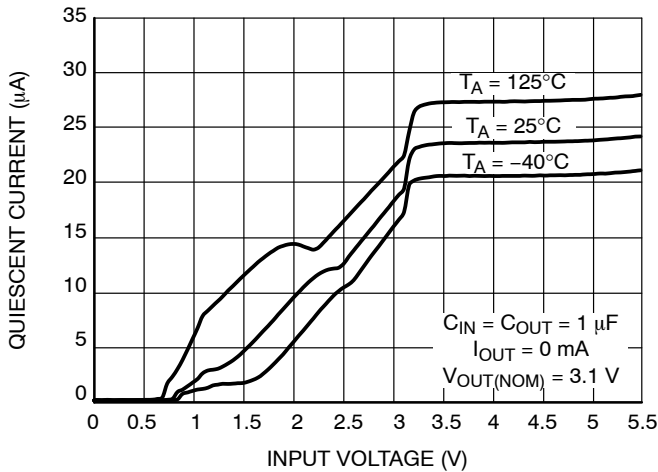
Figure 13. Quiescent Current vs. Input Voltage V_{OUT} = 3.1 V
