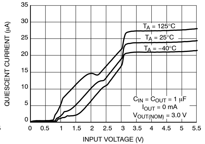
Figure 12. Quiescent Current vs. Input Voltage V_{OUT} = 3.0 V
