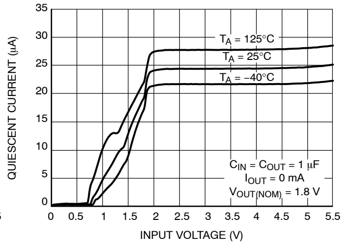
Figure 10. Quiescent Current vs. Input Voltage V_{OUT} = 1.8 V
