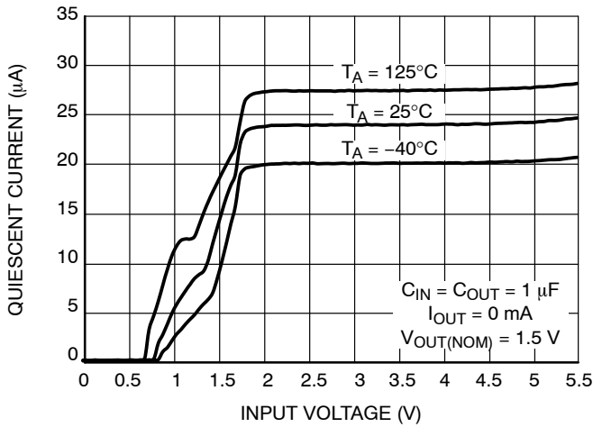
Figure 9. Quiescent Current vs. Input Voltage V_{OUT} = 1.5 V
