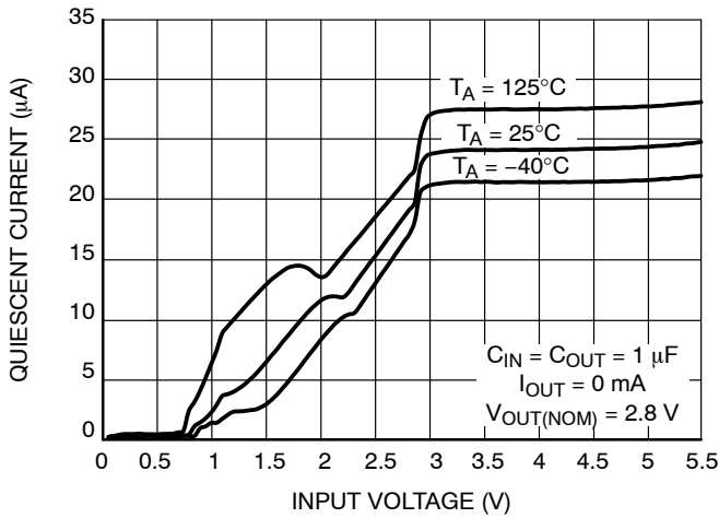
Figure 11. Quiescent Current vs. Input Voltage V_{OUT} = 2.8 V
