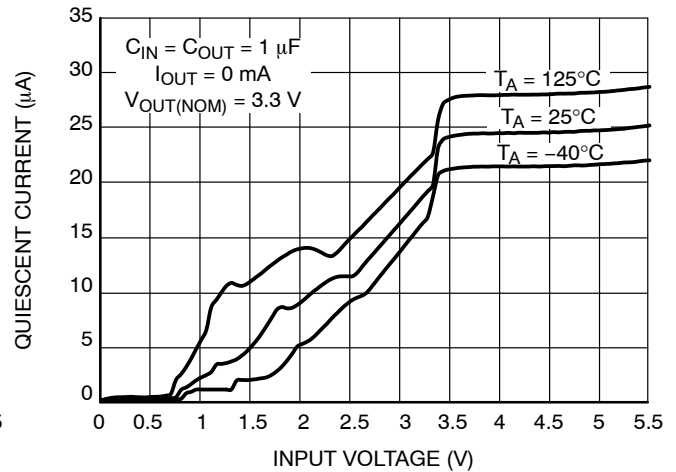
Figure 14. Quiescent Current vs. Input Voltage V_{OUT} = 3.3 V
