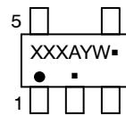
TSOP-5 CASE 483
