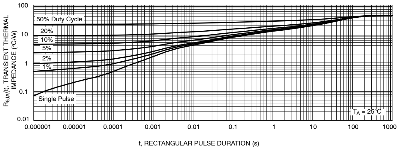
Figure 13. Thermal Characteristics
