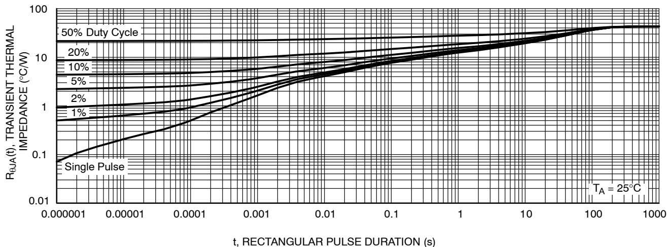
t , RECTANGULAR PULSE DURATION (s)
