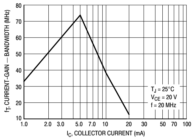
Figure 3. Current-Gain - Bandwidth
