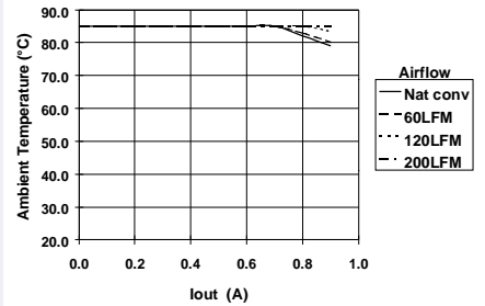
Safe Operating Area @Vin = 24V (Note B)
