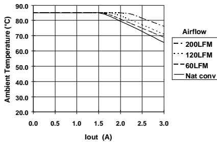
Safe Operating Area @Vin = 24V (Note B)
