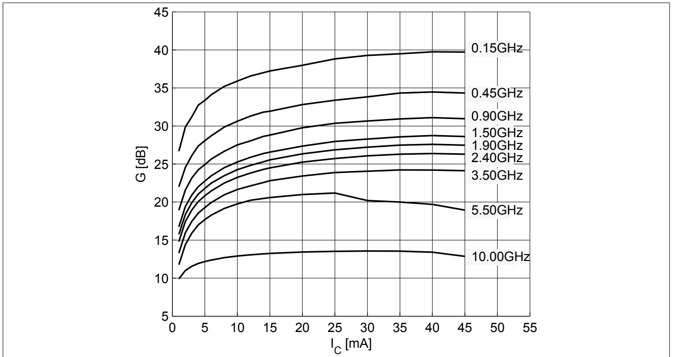
Figure 14 Maximum power gain G_{max} = f(I_C) , V_{CE} = 3 V, f = parameter in GHz
