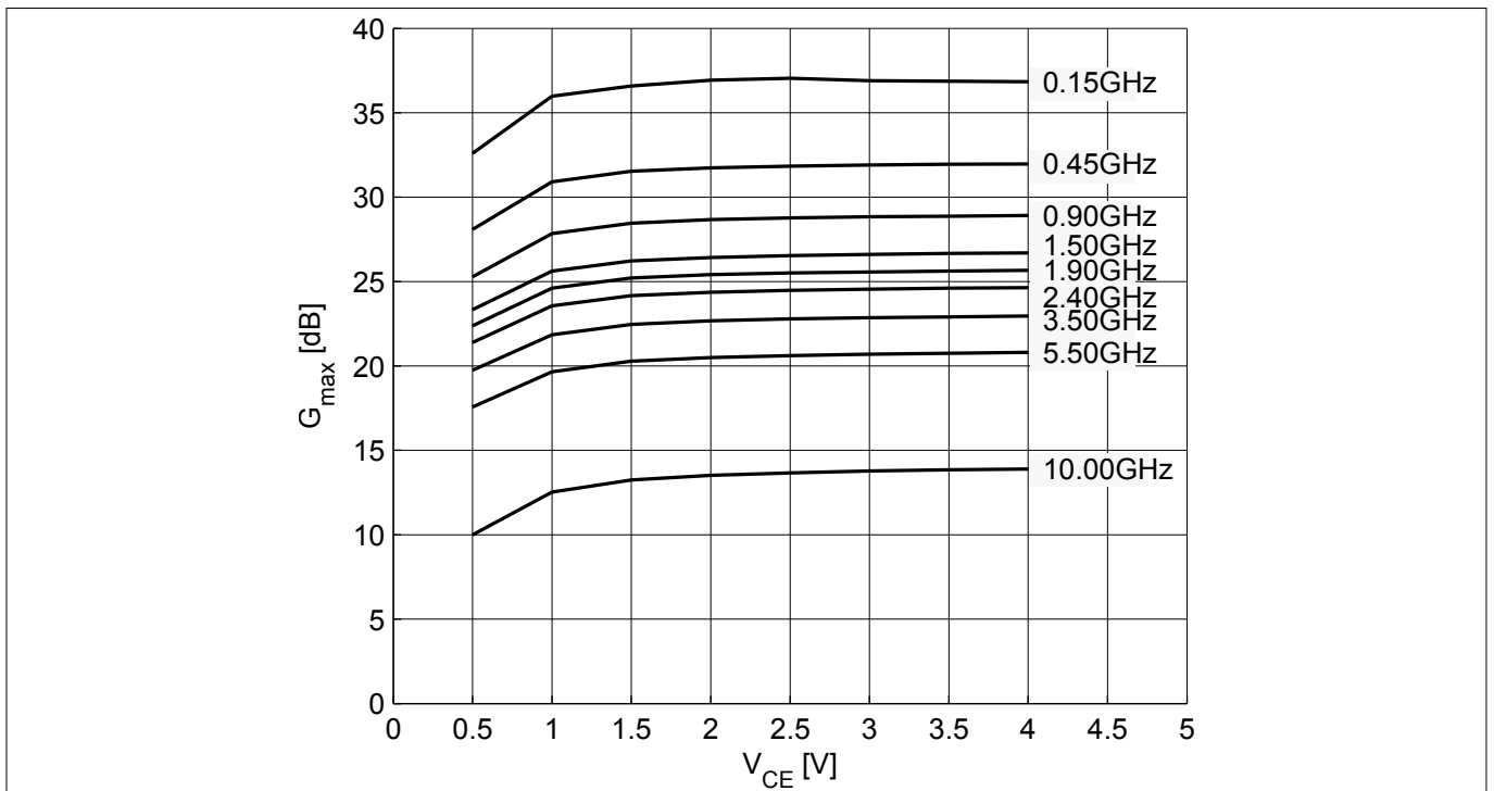
Figure 15 Maximum power gain G_{max} = f(V_{CE}) , I_C = 15 mA, f = parameter in GHz
