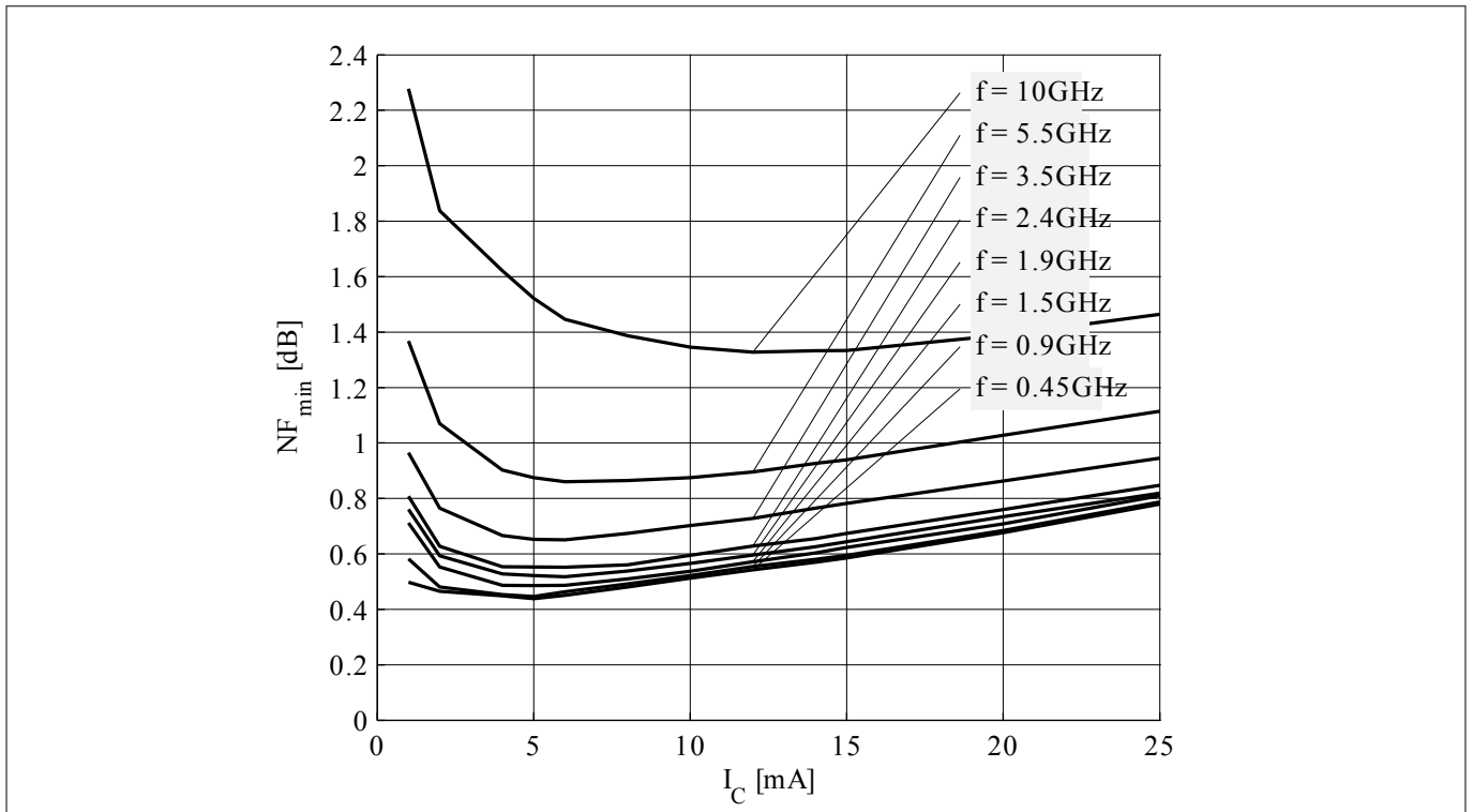
Figure 20 Noise figure NF_{min} = f(I_C) , V_{CE} = 3\text{ V} , Z_S = Z_{S,opt} , f = parameter in GHz
