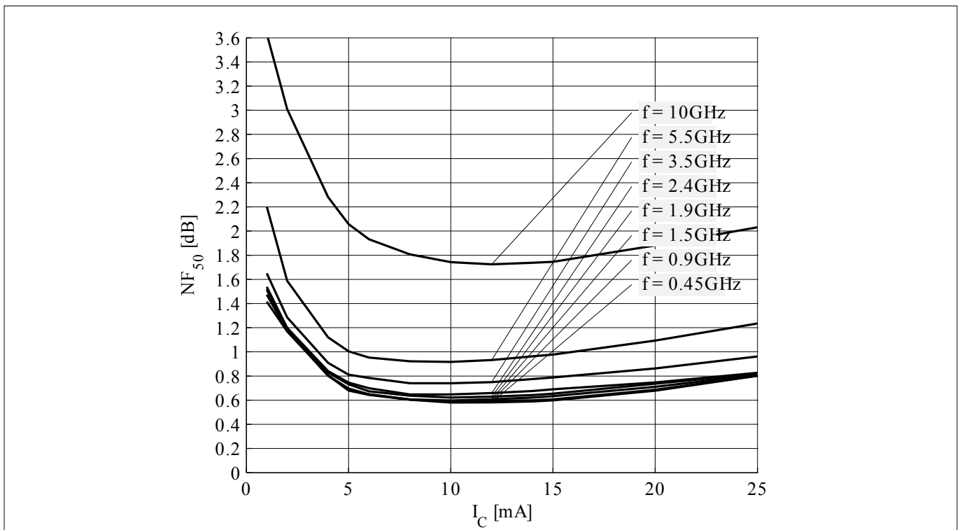
Figure 21 Noise figure NF_{50} = f(I_C) , V_{CE} = 3\text{ V} , Z_S = 50\ \Omega , f = parameter in GHz
