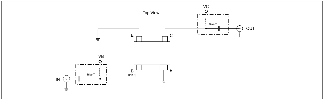
Figure 2 Testing circuit
