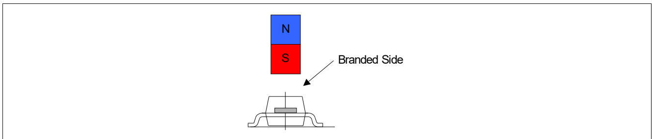
Figure 9 Definition of magnetic field direction PG-SOT23-3-15
